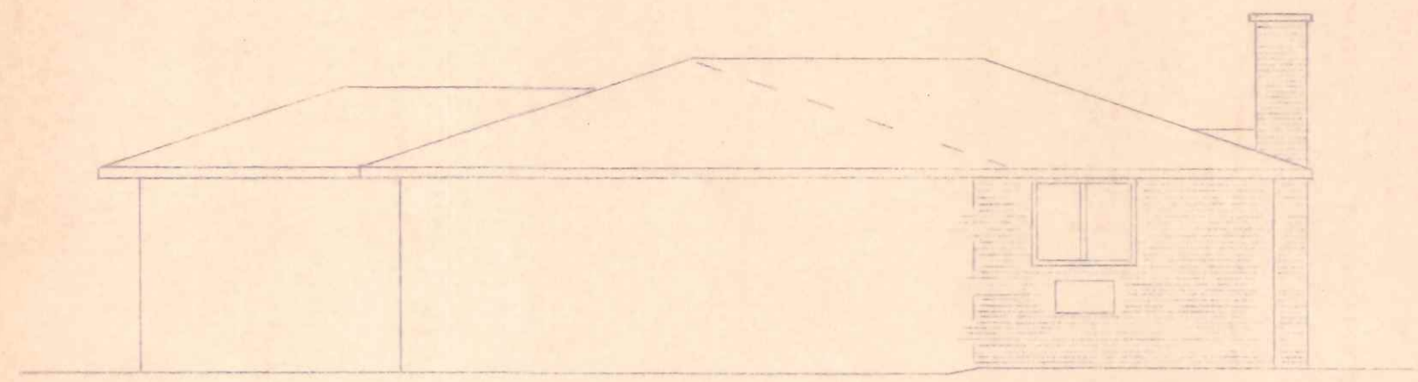
WEST ELEVATION
